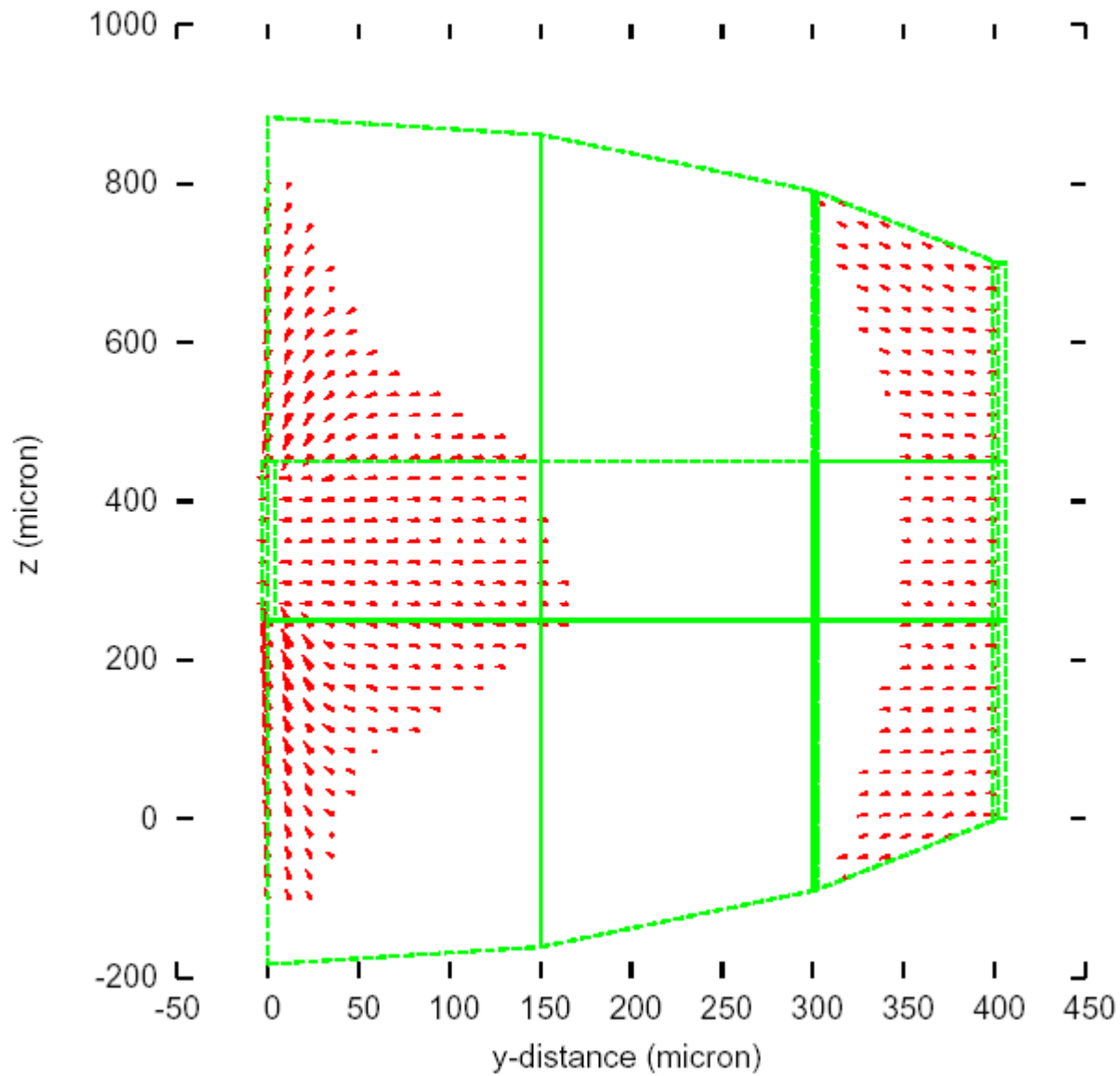
Current flow in the 3D LED structure on y-z plane
