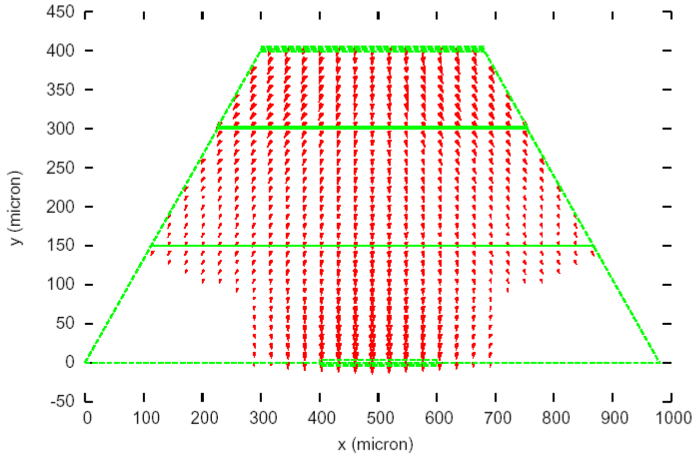
Current flow in a 3D LED structure on x-y plane
